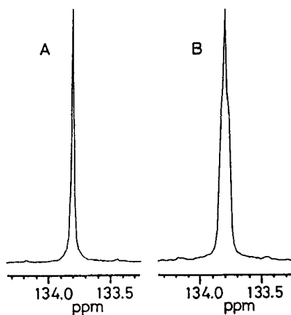
Fig. 1. C4 resonances of [4- ^{13}\text{C} ]BA (A) and [2,4,6,7- ^{13}\text{C}_4 ]BA (B) detected by ^1\text{H} -decoupled ^{13}\text{C} NMR spectroscopy.
